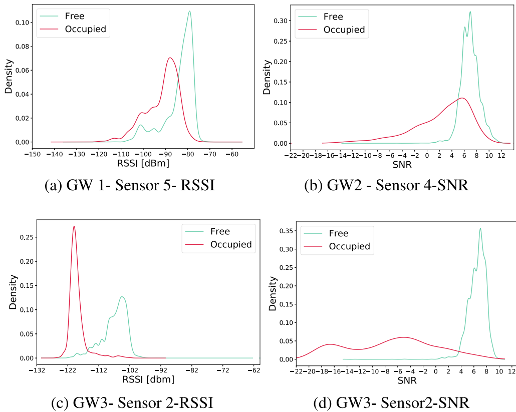
Fig. 8. Probability density function of RSSI and SNR values alterations for diverse sensors and occupancy status from GW1, GW2 and GW3, respectively.
