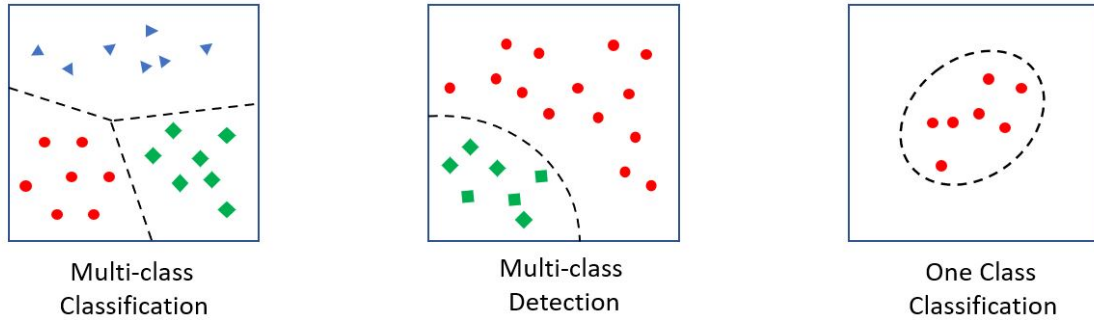
Figure 3.8. One class classification vs multi-class classification/detection [5]
