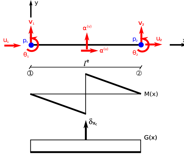
Figure 5.4: The enhanced finite element with it's degrees of freedom and discontinuous shape function M(x) and it's derivative G(x)
