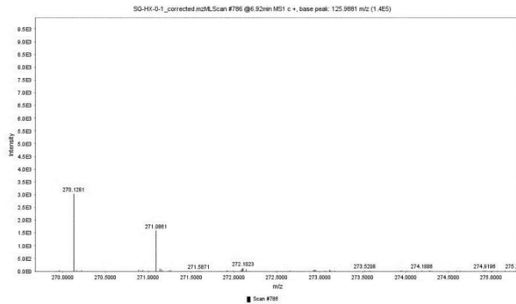
Figure S38. Mass spectrum of strepsilin with m/z 271.0861.
