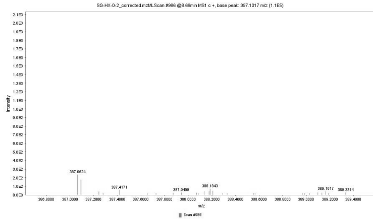
Figure S36. Mass spectrum of stictic acid with m/z 387.0624.
