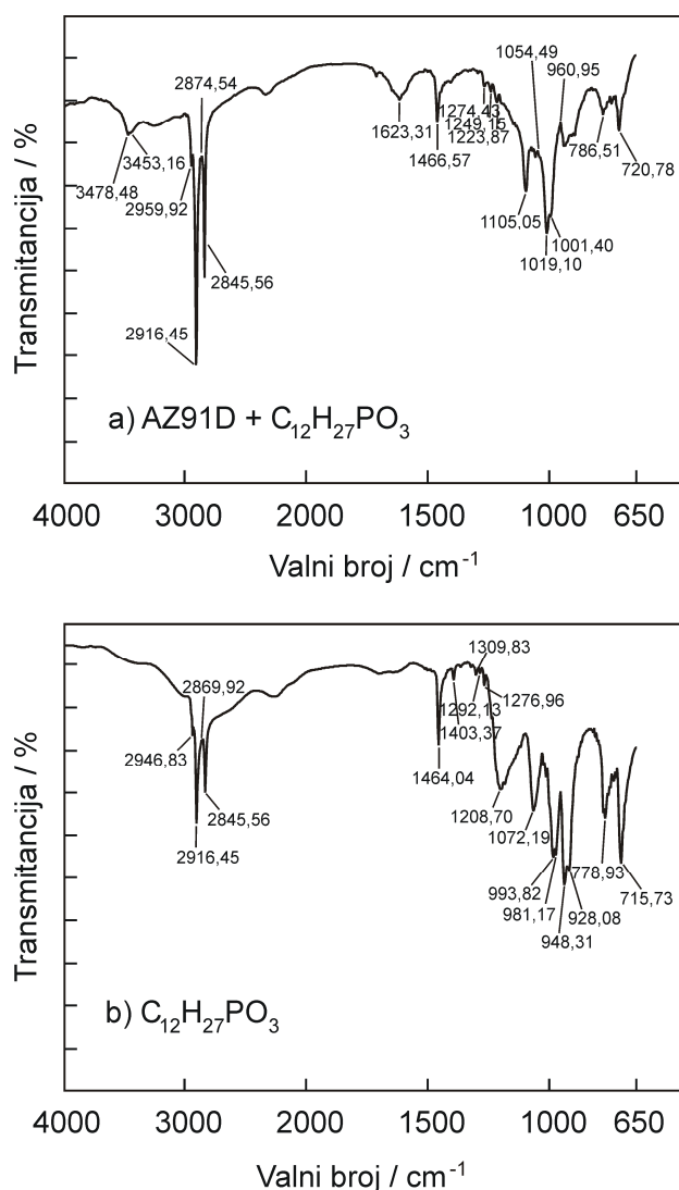
Slika 4.27. (a) FTIR spektar AZ91D legure modificirane SAMom DDPA i (b) FTIR spektar praha DDPA, \text{C}_{12}\text{H}_{37}\text{PO}_3 .
