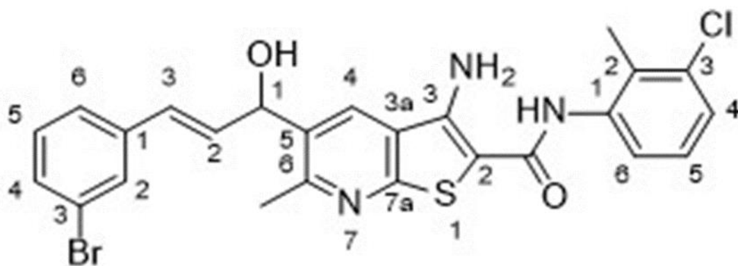
Slika 12. Inhibitor 9 ((E)-3-amino-5-(3-(3-bromophenyl)-1-hydroxyallyl)-N-(3-chloro-2-methylphenyl)-6-methylthieno[2,3-b]pyridine-2-carboxamide)
