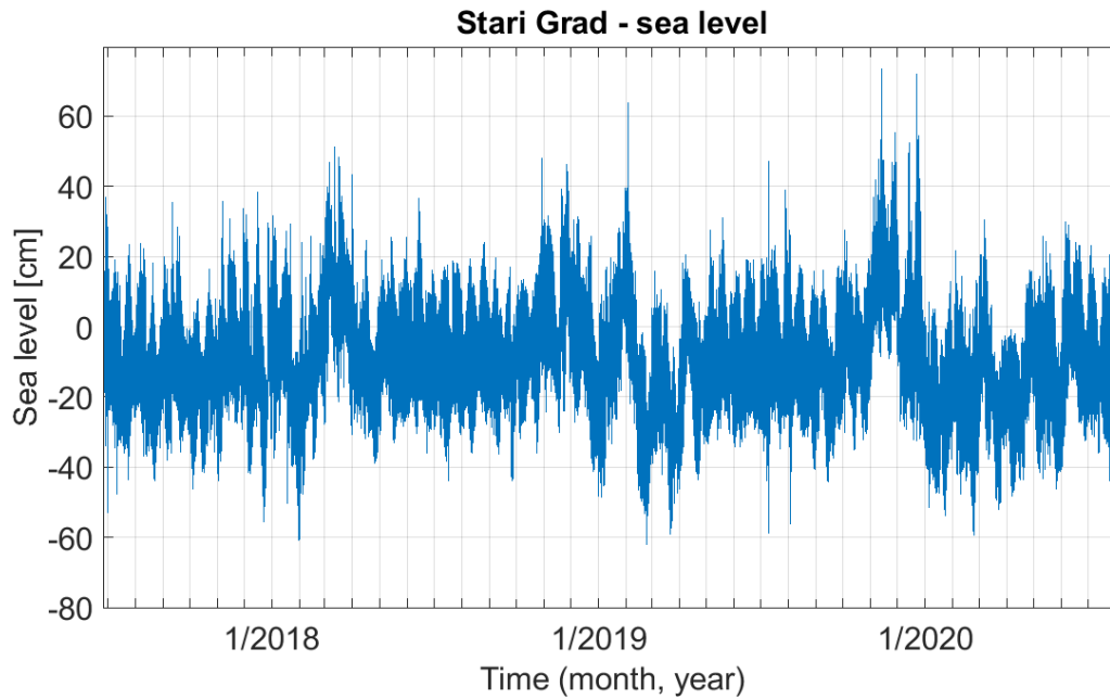
Figure 10. Interpolated sea-level time series.
