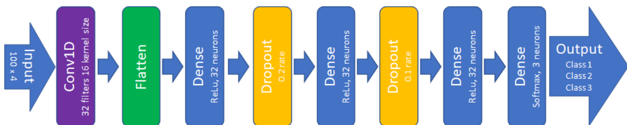
Figure 6. ANN architecture.
