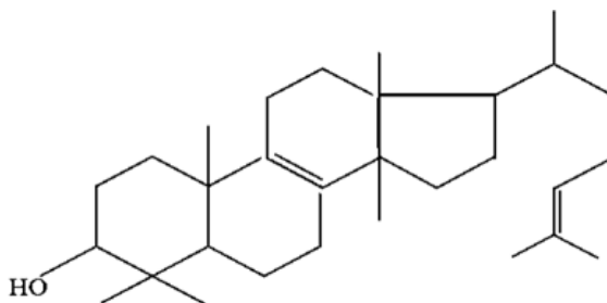
Lanosterol
