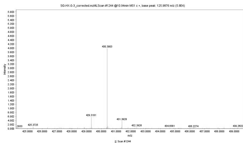
Figure S8. Mass spectrum of cerevisterol with m/z 431.3928.
