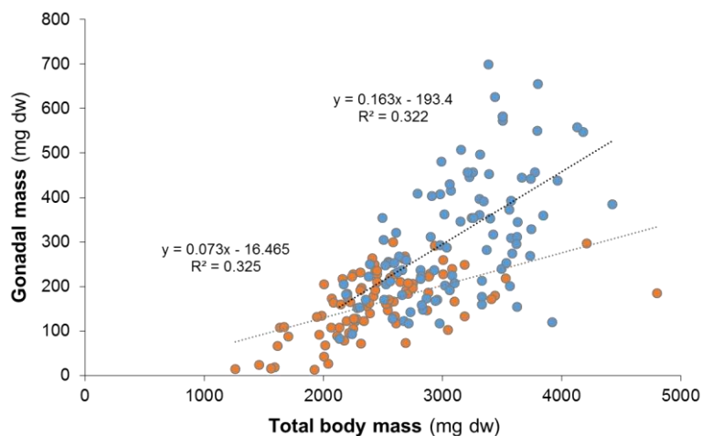
Figure 4.3.7. Relationship between gonadal mass (mg dw) and total body mass (mg dw) before spawning in Pag (blue) and Cetina (orange)
