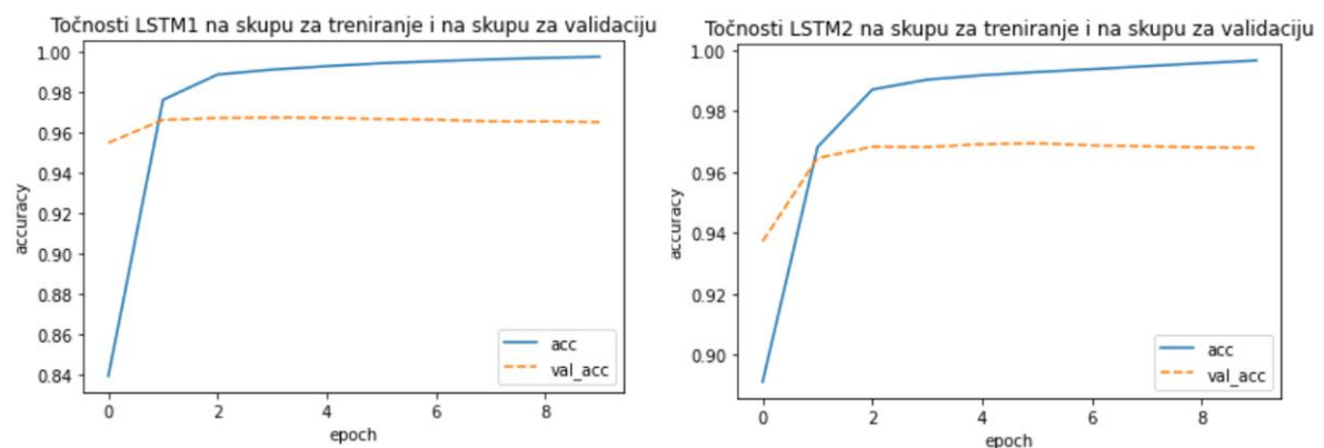
Slika 31 LSTM (acc vs val_acc)
