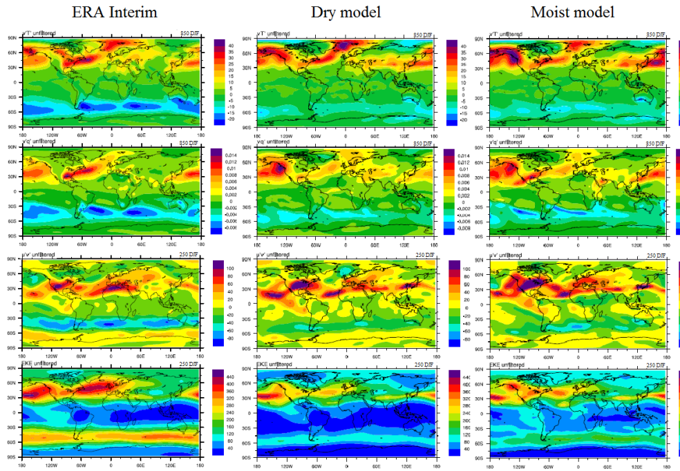
FIGURE 3.3: Unfiltered results for temperature (first row) and humidity (second row) fluxes ( v'T' and v'q' respectively where v' , T' and q' represents anomalies of each variables obtained by subtracting mean value from the series) at lower level and results for momentum flux (third row) and eddy kinetic energy (fourth row) ( u'v' and 1/2[u'^2 + v'^2] respectively) at upper level.
