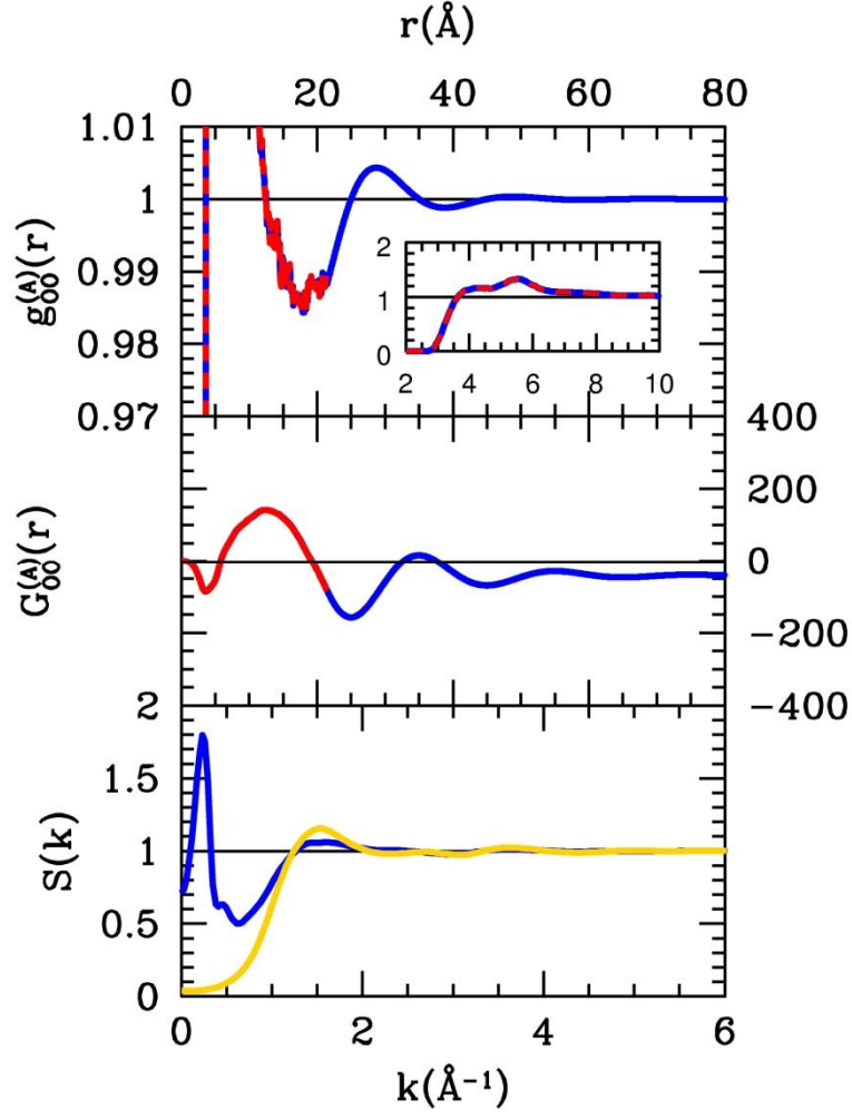
Figure 7.15: Illustration of the TS extension procedure for acetone–acetone correlation function g_{oo}^{(A)}(r) at acetone mole fraction x = 0.30 . The TS parameters are d = 40 \text{ Å} and \xi = 10 \text{ Å} . Colour and line conventions are the same as in Fig. 7.14. Horizontal line is the experimental KBI from Ref. [4]. Bottom panel shows the site–site structure factor of neat TraPPE–UA acetone.
