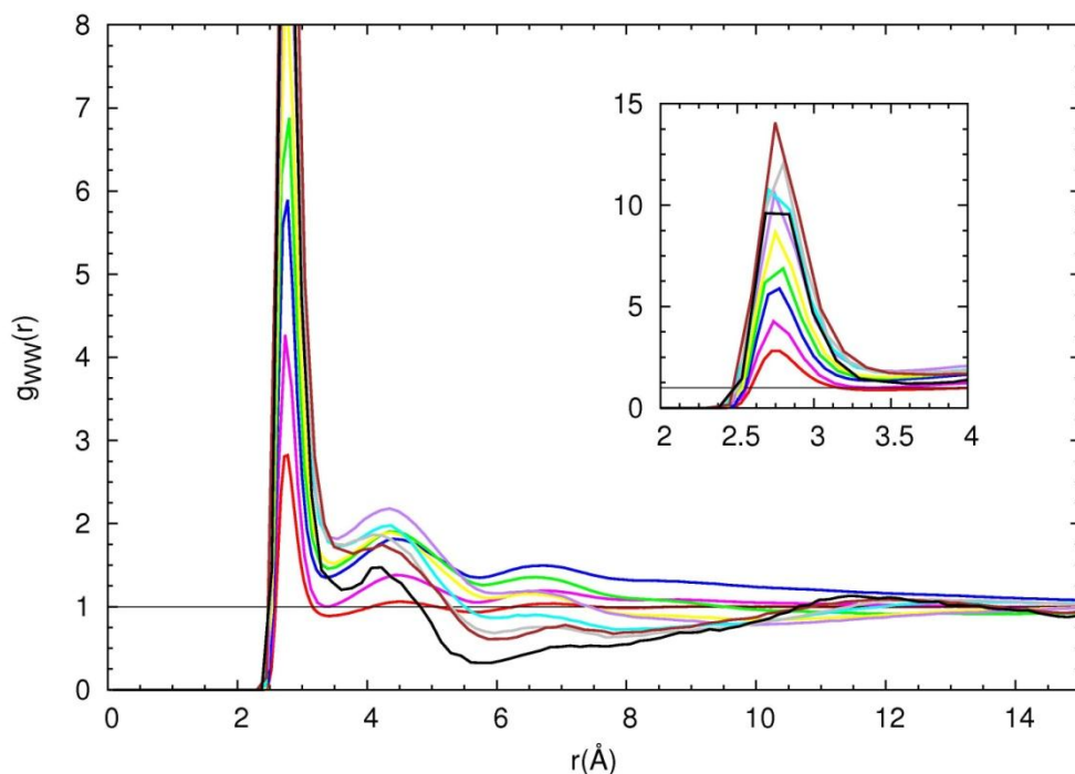
Figure 7.2: Water O–O site distribution functions for OPLS TBA mole fractions from x = 0 (red curve) to x = 0.90 (black curve). Inset shows the zoom on the first peak of the g_{ww}(r) . Colour convention: x = 0.90 (black), x = 0.80 (brown), x = 0.70 (gray), x = 0.60 (cyan), x = 0.50 (purple), x = 0.40 (yellow), x = 0.30 (green), x = 0.20 (blue) and x = 0.10 (magenta).
