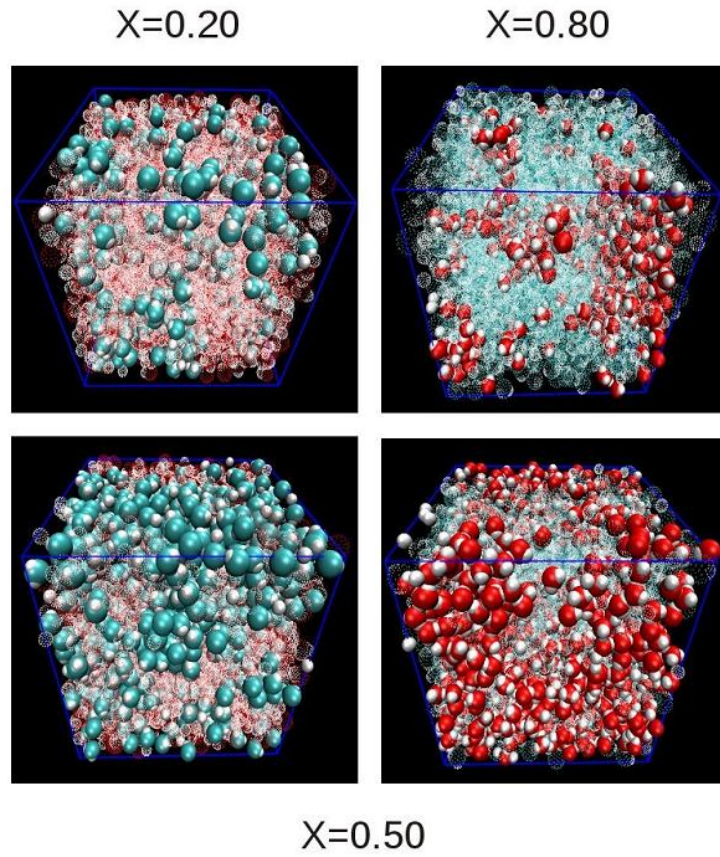
Figure 8.8: Snapshots of the 4/5 model. The colour convention is the same as in Fig. 8.3. Top left panel: x = 0.20 , top right: x = 0.80 , two bottom panels: x = 0.50 , the water and “weak water” molecules are shown in separate shots taken under the same angle.
